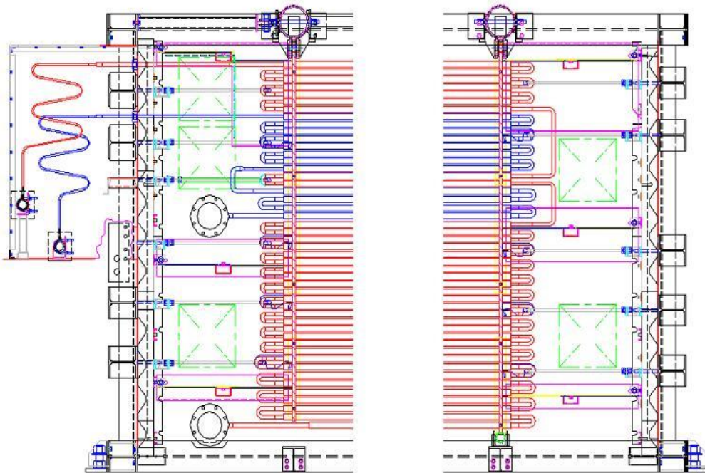
Figure 4: Typical OTSG pressure part module
