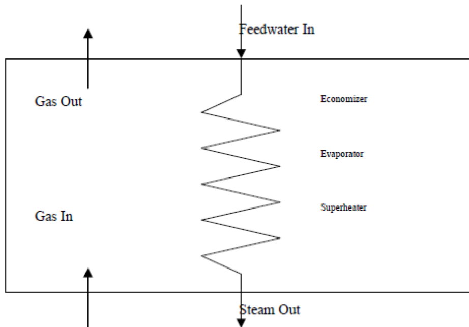
Figure 1: Once Through Steam Generator
