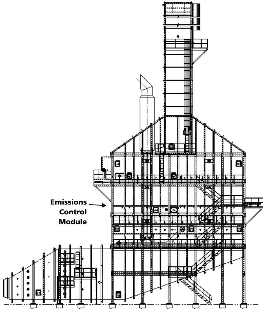
Figure 5: Emissions control module location
