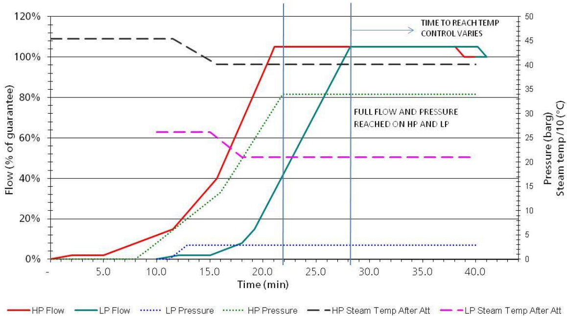
Figure 6: Typical OTSG start-up curve
